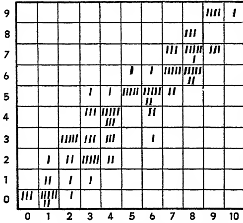
FIG. XV Scatter diagram. Correlation of approximately +0.9 .
